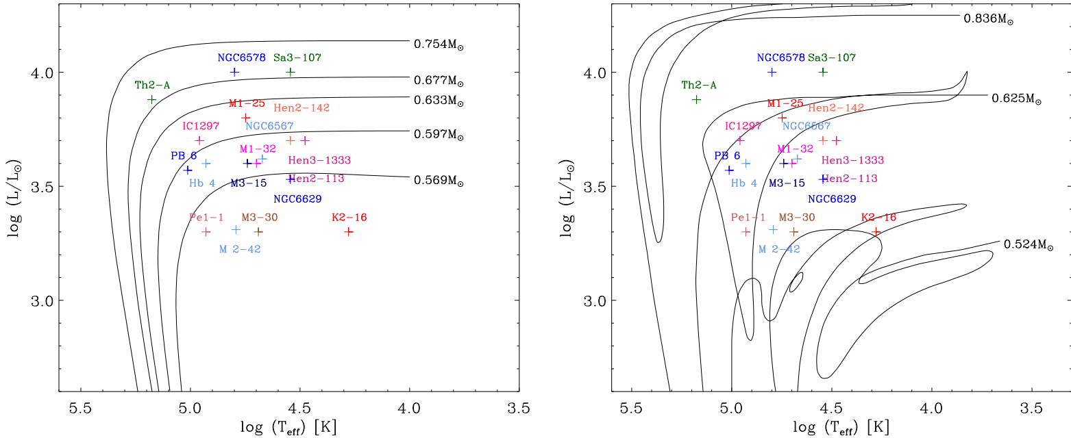
Figure 2.1: Left panel: Positions of the central stars of our sample on the HR diagram for hydrogen-burning models with (M_{\text{ZAMS}}, M_{\star}) = (1M_{\odot}, 0.569M_{\odot}) , (1.5M_{\odot}, 0.597M_{\odot}) , (2M_{\odot}, 0.633M_{\odot}) , (2.5M_{\odot}, 0.677M_{\odot}) and (3M_{\odot}, 0.754M_{\odot}) and metallicity Z = 0.016 from Vassiliadis & Wood (1994). Right panel: Evolutionary tracks for helium-burning models with (M_{\text{ZAMS}}, M_{\star}) = (1M_{\odot}, 0.524M_{\odot}) , (3M_{\odot}, 0.625M_{\odot}) and (5M_{\odot}, 0.836M_{\odot}) from Blöcker (1995a). M_{\text{ZAMS}} is the zero-age main sequence (ZAMS) mass and M_{\star} the final post-AGB mass of the central star.
