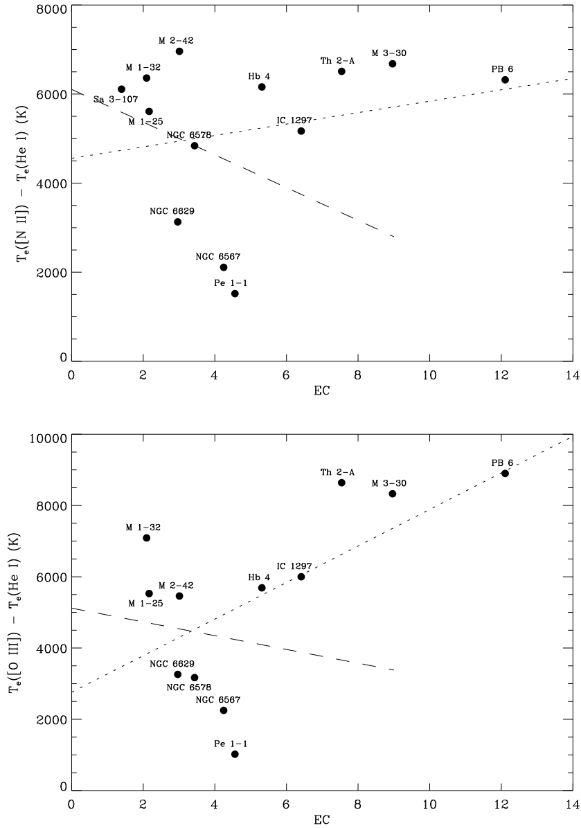
Figure 3.15: Top panel: the difference \Delta T_e (K) between the nebular electron temperatures derived from the [N II] CELs, T_e([N II]) , and from the He I ORLs, T_e(\text{He I}) , plotted against the excitation class (EC). Bottom panel: the difference \Delta T_{[O III]} (K) between the nebular [O III] electron temperatures, T_e([O III]) , and the He I temperatures, T_e(\text{He I}) , plotted against the EC. The dotted line is a linear fit to \Delta T_e as a function of EC. The dashed line is a similar linear fit found after excluding PB 6, M 3-30 and Th 2-A, discussed in the text.
