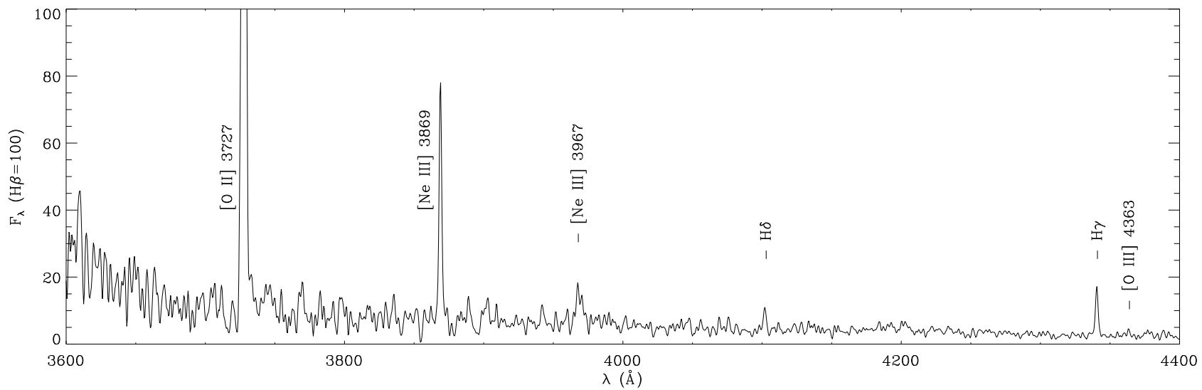
Figure 7.2: The observed optical spectrum from an aperture 10'' \times 20'' taken from field 2 located on the east ring of the PN SuWt 2 and normalized such that F(\text{H}\beta) = 100 : blue spectra (top) covers wavelengths 3600–4400 Å and red spectra (middle and bottom) covers 4400–8000 Å.
