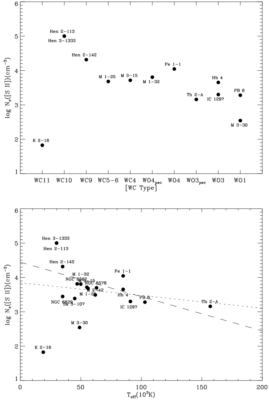
Figure 3.4: Top panel: variation of the logarithmic electron density \log N_e([S II]) ( \text{cm}^{-3} ) along the spectral sequence. Bottom panel: variation of the logarithmic electron density \log N_e([S II]) ( \text{cm}^{-3} ) along the stellar effective temperature T_{\text{eff}} ( 10^3 \text{ K} ). The dotted line is a linear fit to \log N_e([S II]) as a function of T_{\text{eff}} . The dashed line is a similar linear fit found after excluding K 2-16 and M 3-30, discussed in the text.
