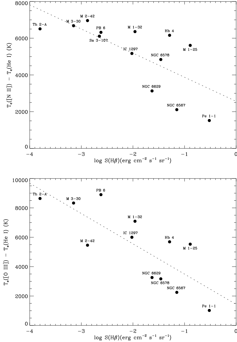
Figure 3.13: Top panel: the difference \Delta T_{[\text{N II}]} (\text{K}) between the nebular electron temperatures derived from the [\text{N II}] CELs, T_e([\text{N II}]) , and from the He I ORLs, T_e(\text{He I}) , plotted against the logarithmic intrinsic nebular \text{H}\beta surface brightness \log S(\text{H}\beta) (\text{erg cm}^{-2} \text{s}^{-1} \text{sr}^{-1}) . The dotted line is a linear fit to \Delta T_{[\text{N II}]} as a function of \log S(\text{H}\beta) . Bottom panel: the difference \Delta T_{[\text{O III}]} (\text{K}) between the nebular [\text{O III}] electron temperatures, T_e([\text{O III}]) , and the He I temperatures, T_e(\text{He I}) , plotted against \log S(\text{H}\beta) . The dotted line is a linear fit to \Delta T as a function of \log S(\text{H}\beta) , discussed in the text.
