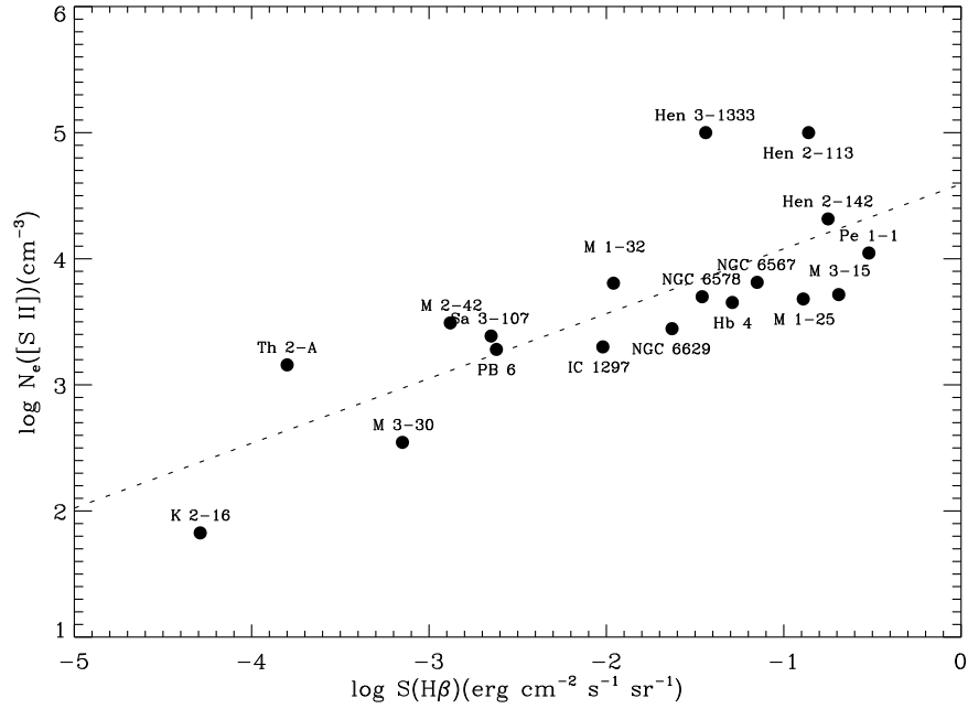
Figure 3.5: The logarithmic electron density \log N_e([S II])(\text{cm}^{-3}) plotted against the logarithmic intrinsic nebular H\beta surface brightness \log S(H\beta)(\text{erg cm}^{-2} \text{s}^{-1} \text{sr}^{-1}) . The dotted line is a linear fit to \log N_e([S II]) as a function of \log S(H\beta) , discussed in the text.
