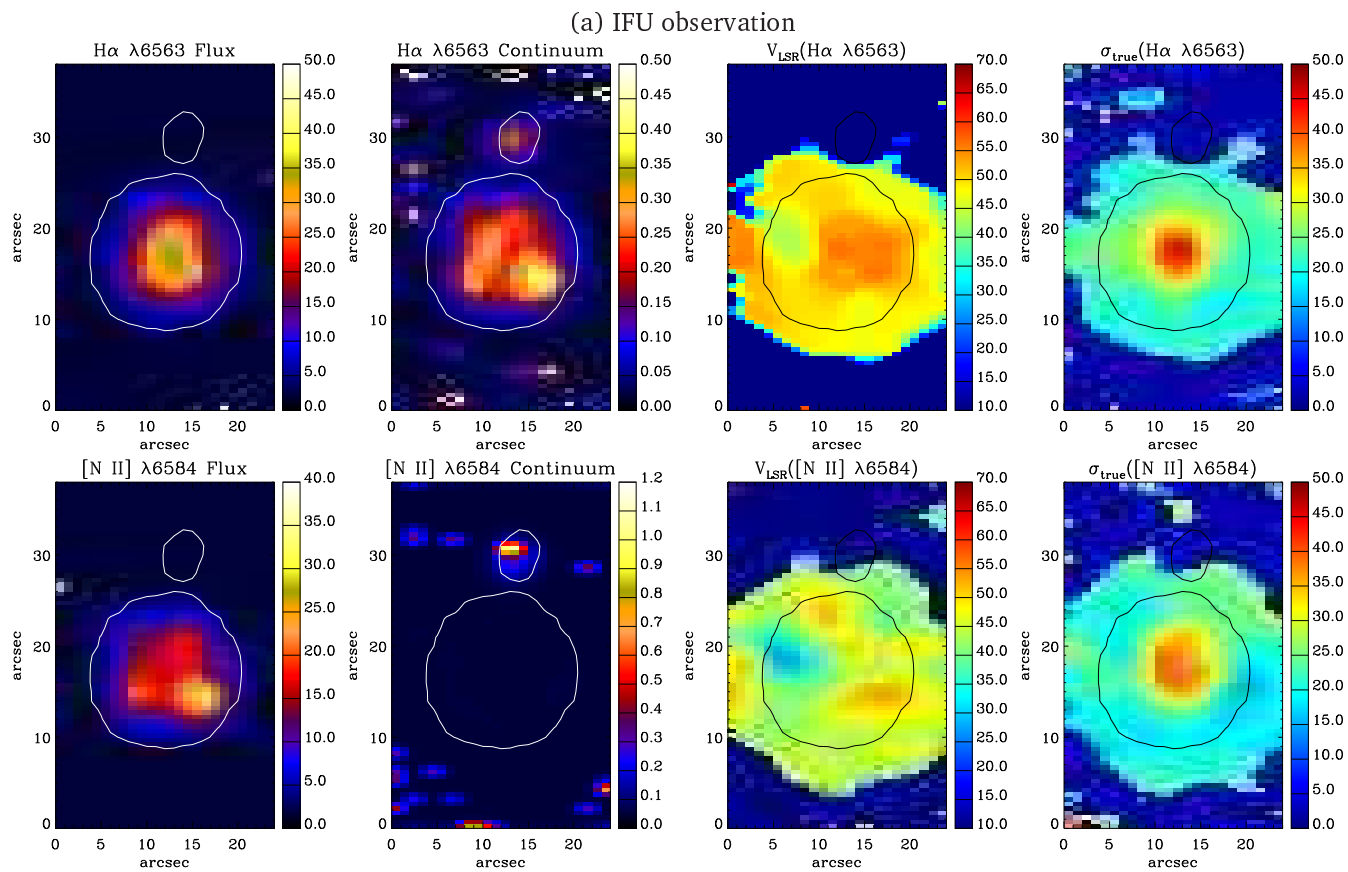
Figure A.1: (a) Kinematic maps of PB 6 in H \alpha \lambda 6563 Å (top) and [N II] \lambda 6584 Å (bottom). From left to right: spatial distribution maps of flux intensity, continuum, LSR velocity and velocity dispersion. Flux unit is in 10^{-15} \text{ erg s}^{-1} \text{ cm}^{-2} \text{ spaxel}^{-1} , continuum in 10^{-15} \text{ erg s}^{-1} \text{ cm}^{-2} \text{ Å}^{-1} \text{ spaxel}^{-1} , and velocity unit in \text{km s}^{-1} . North is up and east is toward the left-hand side. White/black contour lines show the distribution of the narrow-band emission of H \alpha in arbitrary unit obtained from the SHS. (b) The STIS/MIRVIS filter image taken by the Hubble Space Telescope (HST; Observing program 12600; PI. Dufour, 2012).
