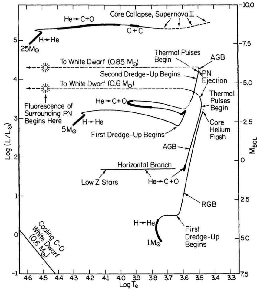
Figure 1.2: Stellar evolutionary tracks for stars with initial masses of 1, 5 and 25M_{\odot} . The stellar luminosity unit in the solar luminosity L_{\odot} and the effective temperature unit in Kelvine. The nuclear burning phases are labeled. From Iben (1995)
