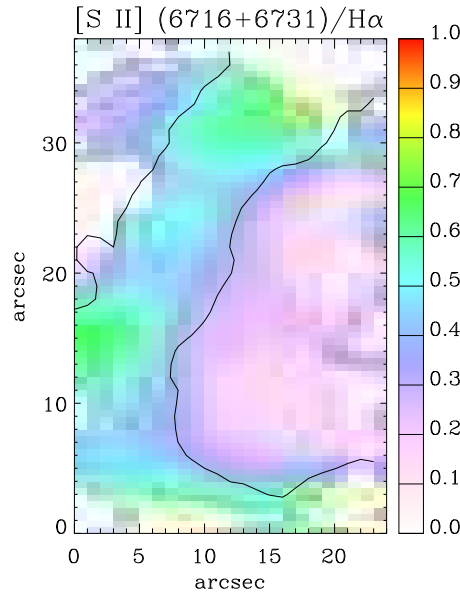
Figure 7.5: Flux ratio maps of the [\text{S II}] \lambda 6716+6731 \text{ \AA} to the \text{H}\alpha recombination line emission.
