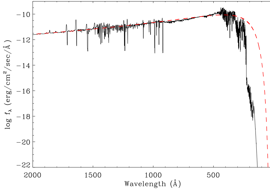
Figure 5.5: Non-LTE model atmosphere flux (solid line) calculated with the PoWR models for the surface abundances \text{H:He:C:N:O} = 10:85:0.3:5:0.6 by mass and the stellar temperature T_{\text{eff}} = 70 \text{ kK} (Todt et al. 2013), compared with a blackbody (dashed line) at the same temperature.
