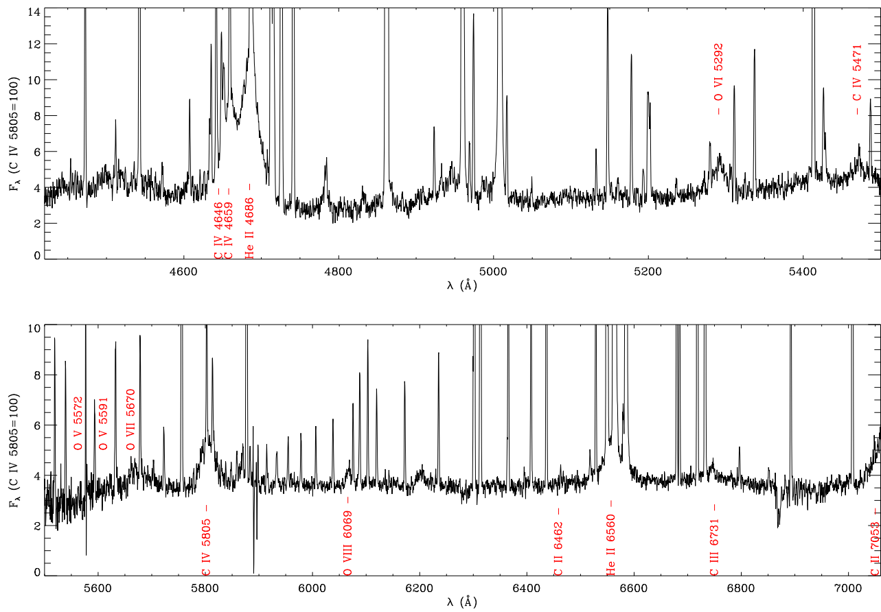
Figure E.1: The observed optical spectra of the CSPN PB 6 and normalized such that F(\text{CIV}5805) = 100 : grating B7000 (top) covers wavelengths 4415–5500 Å and R7000 (bottom) covers 5500–7060 Å.
