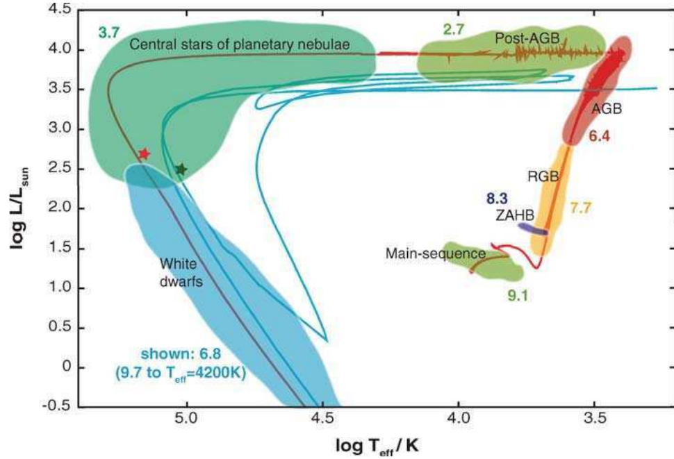
Figure 1.1: Evolutionary tracks of a progenitor star with an initial mass of 2M_{\odot} and solar metallicity shown in the Hertzsprung-Russell diagram. The red track shows a normal evolution phase without any late thermal pulse. The blue track shows a born-again event triggered by a very late thermal pulse. The red star shows the position of the H-deficient central stars of the planetary nebula PG 1159-035, and the green star shows the position of the H-normal central stars of the planetary nebula NGC 6853. The number labels indicate the log of the approximate duration of each evolutionary phase in units of 10^3 yr. From Herwig (2005).
