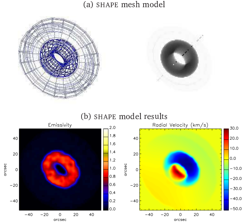
Figure 5.3: (a) The SHAPE mesh model before rendering at the best-fitting inclination and corresponding rendered model. (b) The normalized synthetic intensity map and the radial velocity map at the inclination of -35^\circ and the position angle of 135^\circ , derived from the model ( v_{\text{sys}} = 0 ), which can be compared directly with Fig. 5.2.
