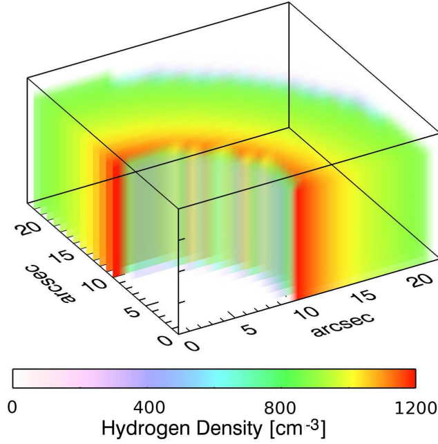
Figure 5.6: The density distribution based on the ISW models adopted for photoionization modelling of Abell 48. The cylinder has outer radius of 23'' and thickness of 13'' . Axis units are arcsec, where 1 \text{ arcsec} is equal to 9.30 \times 10^{-3} \text{ pc} based on the distance determined by our photoionization models.
