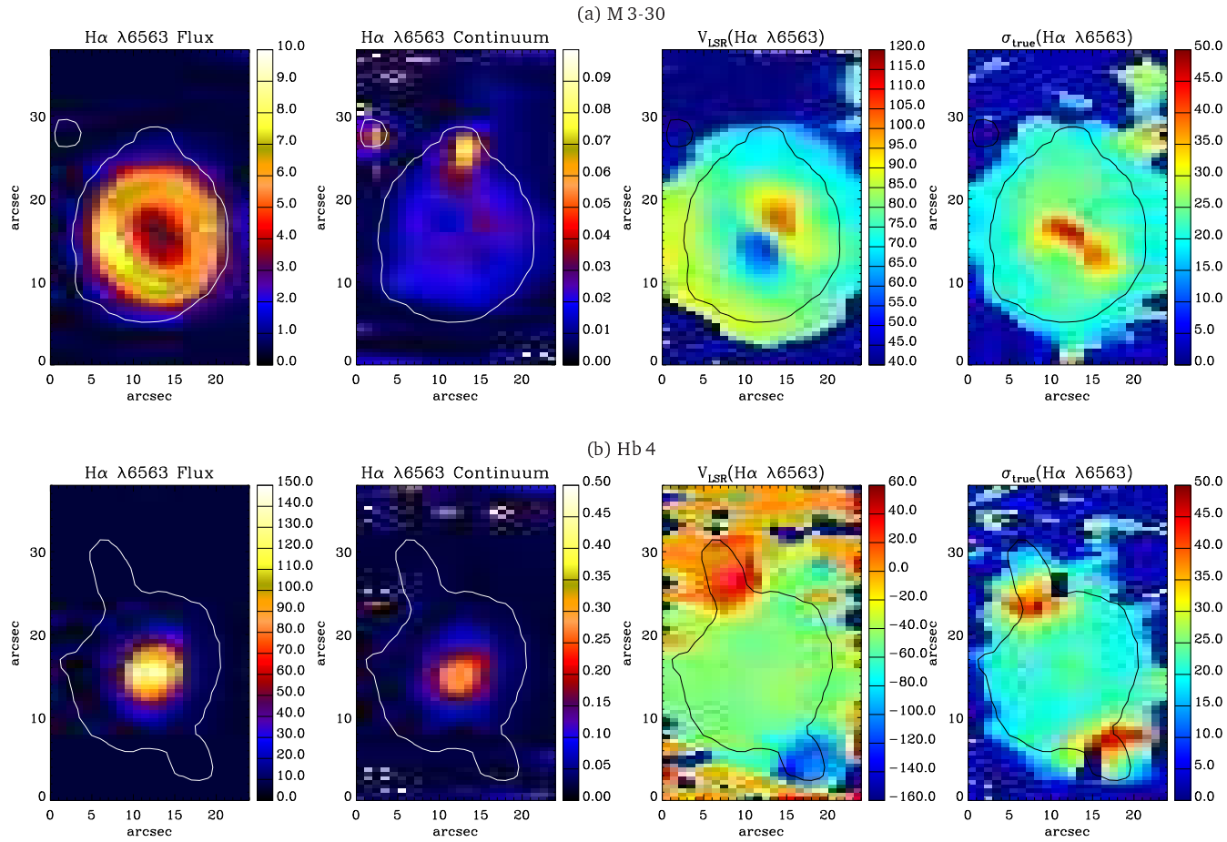
Figure 2.4: From left to right, spatial distribution maps of flux intensity, continuum, LSR velocity and velocity dispersion of H \alpha \lambda 6563 emission line profile for M 3-30, Hb 4, IC 1297, Th 2-A and K 2-16. Flux unit is in 10^{-15} \text{ erg s}^{-1} \text{ cm}^{-2} \text{ spaxel}^{-1} and velocity unit in \text{km s}^{-1} .
