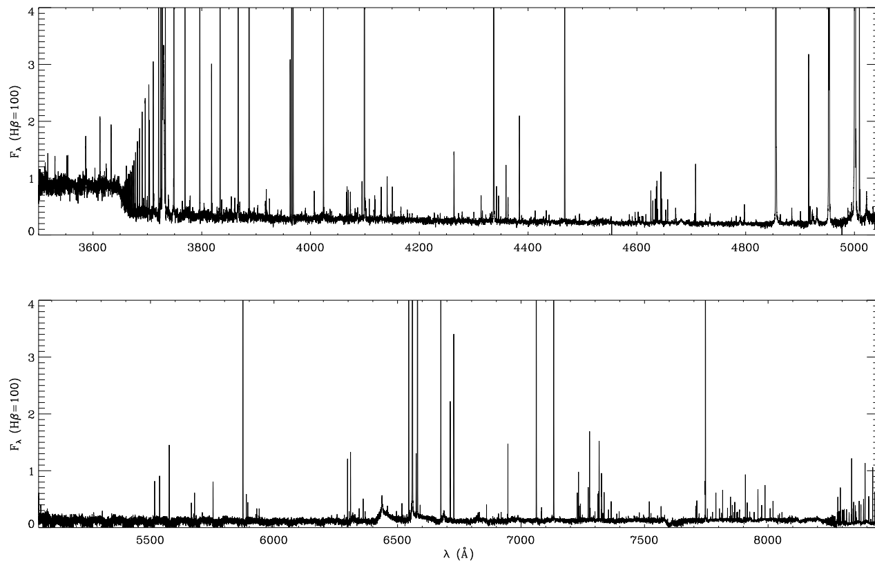
Figure 6.1: The observed optical spectrum of the PN PB 8, covering wavelengths of (top) 3500–5046 Å and (bottom) 5047–8451 Å, and normalized such that F(\text{H}\beta) = 100 (García-Rojas et al. 2009).
