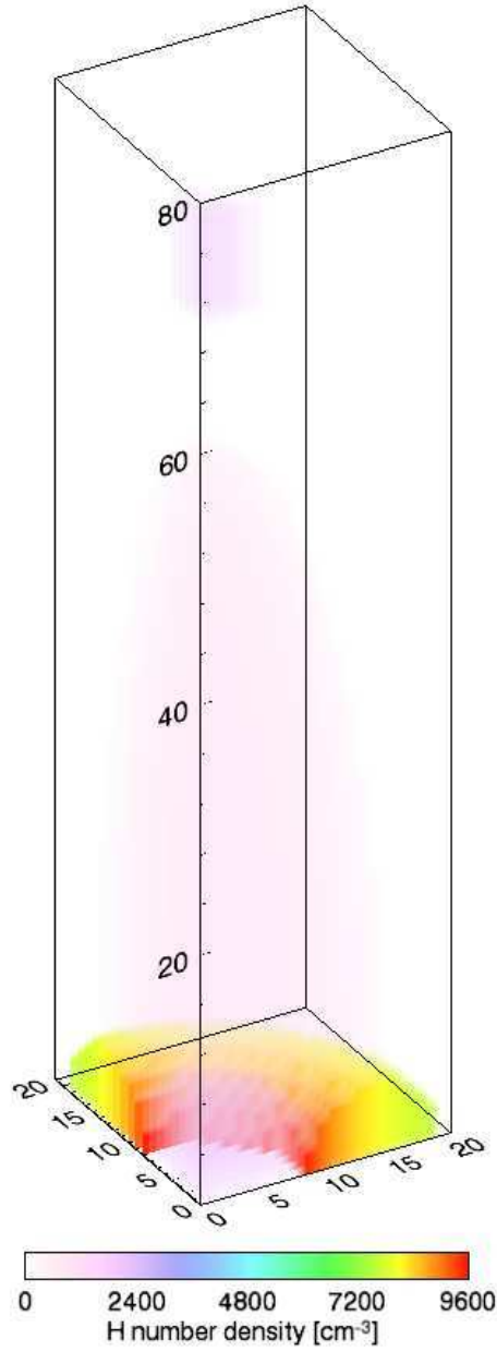
Figure 4.4: The density distribution constructed in 20 \times 20 \times 80 cubic grids adopted for photoionization modeling of Hb 4. Each cubic cell has a length of 1.0 \times 10^{16} cm. The torus has a power-law density distribution, a radius of 1.4 \times 10^{17} cm from its center to the tube center, and a tube radius of 6.0 \times 10^{16} cm. The FLIER is a cylinder with a radius of 5 \times 10^{16} cm and a length of 1.0 \times 10^{17} cm, and is located at the distance of 7.0 \times 10^{17} cm from the center of the torus. The outer halo is an ellipsoid with a semimajor axis of 6.0 \times 10^{17} cm and a semiminor axis of 1.5 \times 10^{17} cm. The ionizing source is placed in the corner (0,0,0).
