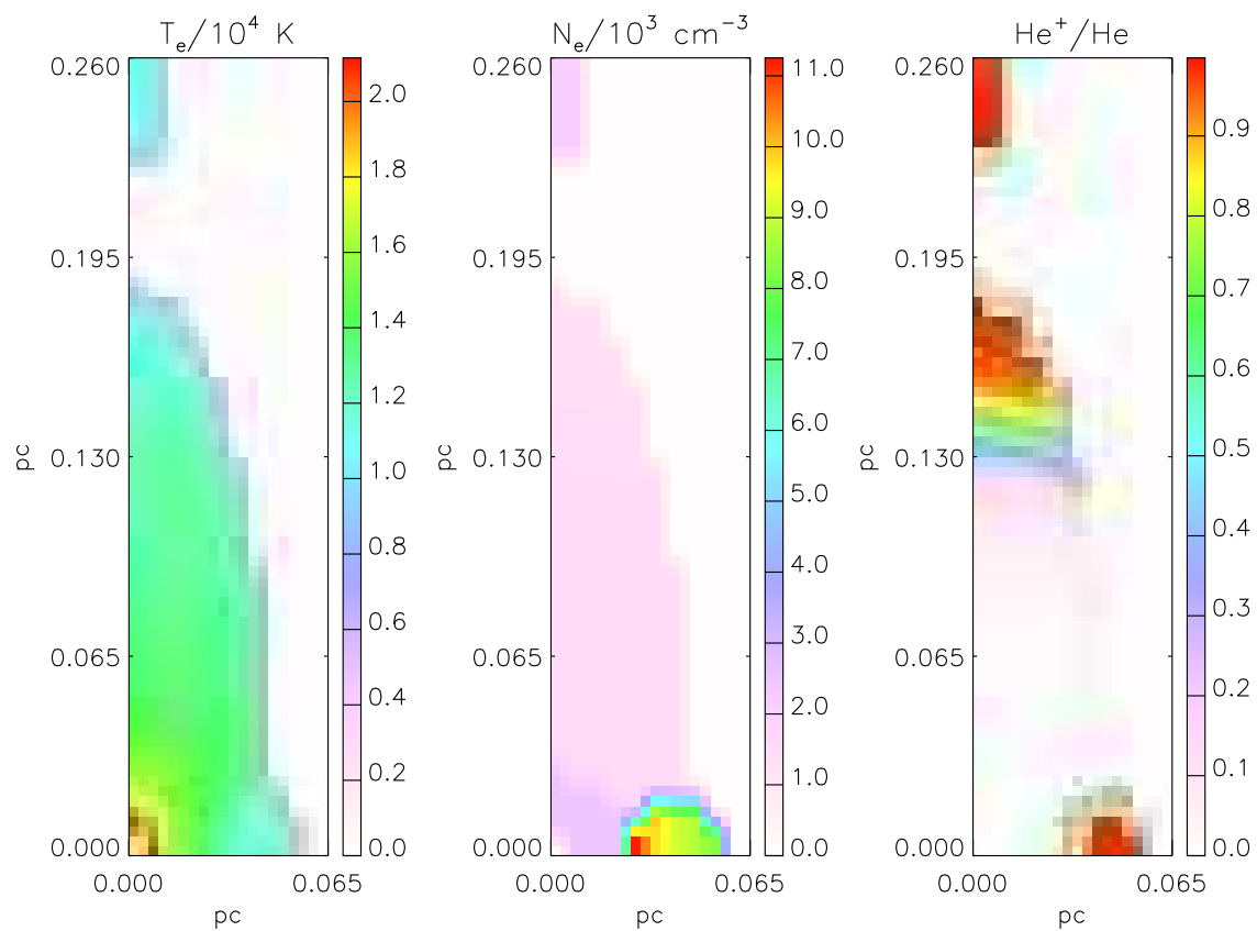
Figure 4.6: Spatial distributions of electron temperature, electron density and ionic fractions from the photoionization MC1. Ionic fractions are shown for \text{He}^+ , \text{He}^{2+} , \text{N}^+ , \text{N}^{2+} , \text{O}^+ , \text{O}^{2+} and \text{S}^+ . The ionizing source is placed in the corner (0,0,0).
