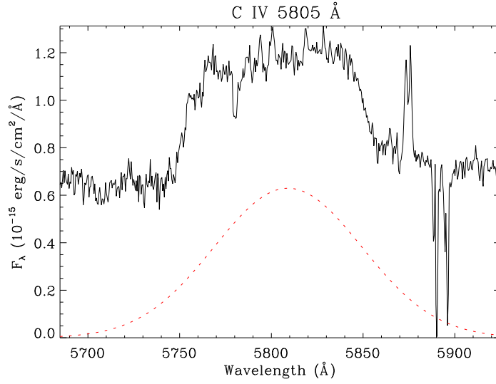
Figure 1.12: The C IV-5801/12 doublet line profile of the central star [WO 3] pec of Th 2-A. The dotted line (red color) shows the Gaussian component that best-fits the observed line profile (black solid line).
