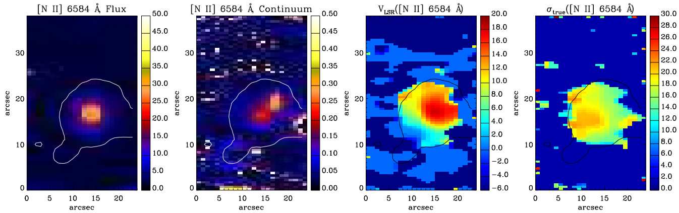
Figure 6.2: Maps of PB 8 in [N II] \lambda 6584 \text{ \AA} from the IFU observation. From left to right: spatial distribution maps of flux intensity, continuum, LSR velocity and velocity dispersion. Flux unit is in 10^{-15} \text{ erg s}^{-1} \text{ cm}^{-2} \text{ spaxel}^{-1} , continuum in 10^{-15} \text{ erg s}^{-1} \text{ cm}^{-2} \text{ \AA}^{-1} \text{ spaxel}^{-1} , and velocities in \text{km s}^{-1} . North is up and east is toward the left-hand side. The white/black contour lines show the distribution of the narrow-band emission of H \alpha in arbitrary unit obtained from the SuperCOSMOS Sky H \alpha Survey (Parker et al. 2005).
