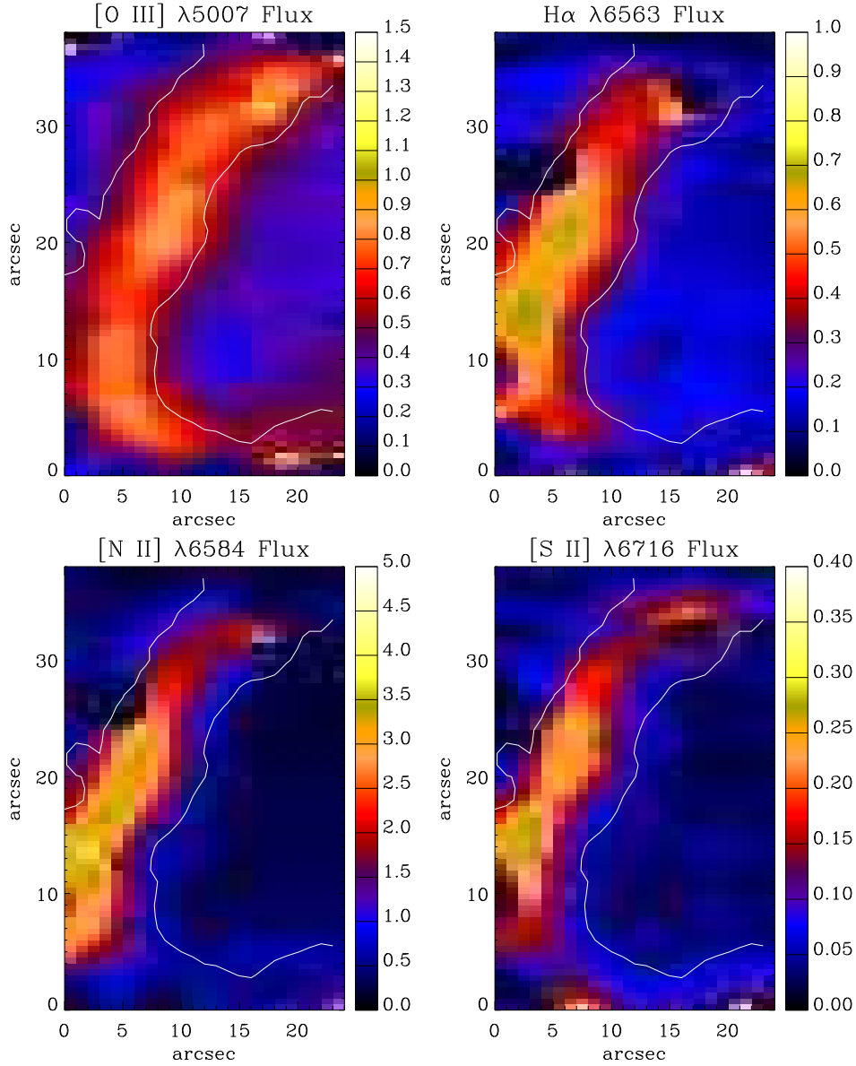
Figure 7.3: Underreddened flux maps for Field 2 (see Fig. 7.1) of the PN SuWt 2: [O III] \lambda 5007 \text{ \AA} , H \alpha \lambda 6563 \text{ \AA} , [N II] \lambda 6584 \text{ \AA} and [S II] \lambda 6716 \text{ \AA} . The flux is derived from single Gaussian profile fits to the emission line at each spaxel. White contour lines show the distribution of the narrow-band emission of H \alpha and [N II] in arbitrary unit taken with the ESO 3.6-m telescope. North is up and east is toward the left-hand side. Flux unit is in 10^{-15} \text{ erg s}^{-1} \text{ cm}^{-2} \text{ spaxel}^{-1} .
