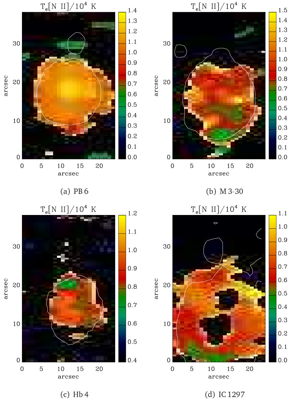
Figure 3.8: As Figure 3.2 but for spatial distribution maps of electron temperature T_e/10^4 (K) from the flux ratio [N II] (6548+6584)/5755 . The white contour lines show the distribution of the narrow-band emission of H\alpha in arbitrary unit obtained from the SHS.
