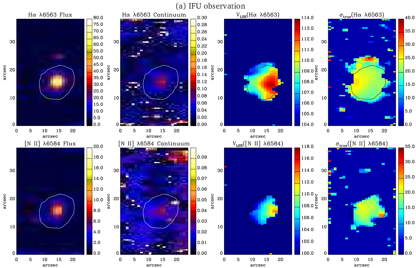
Figure A.8: (a) As Figure A.1 but for M 3-15. (b) The SHAPE mesh model before rendering at the best-fitting inclination, two different orientations (inclination: 90^\circ and 0^\circ , respectively), and corresponding rendered model. (c) The HST image taken by F656N filters (Observing program 9356; PI. Zijlstra, 2002).
