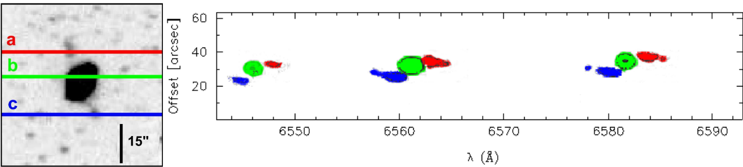
Figure 4.2: Left panel: Deep H\alpha + [\text{N II}] imagery of Hb 4 obtained with MES-SPM and the positions of the three SPM long-slits. Right panel: Long-slit H\alpha + [\text{N II}] spectra of Hb 4 acquired with MES-SPM for slits a (red), b (green) and c (blue).
