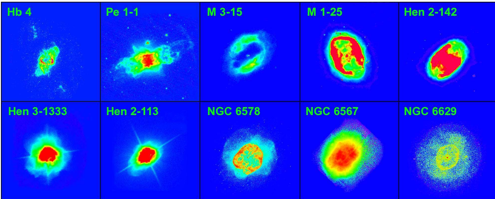
Figure 2.2: HST images of Hb4, Pe 1-1, M 3-15, M 1-25, Hen 2-142, Hen 3-1333, Hen 2-113, NGC 6578, NGC 6567 and NGC 6629. North is up and east is toward the left-hand side. For more detail about the instrument and filter/grating used in each image, see Table 2.2.
