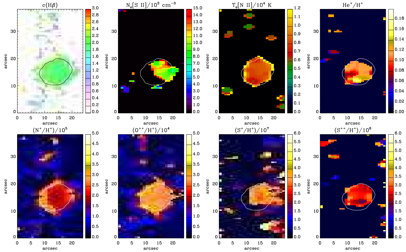
Figure D.6: As Figure D.1 but for Pe 1-1.
