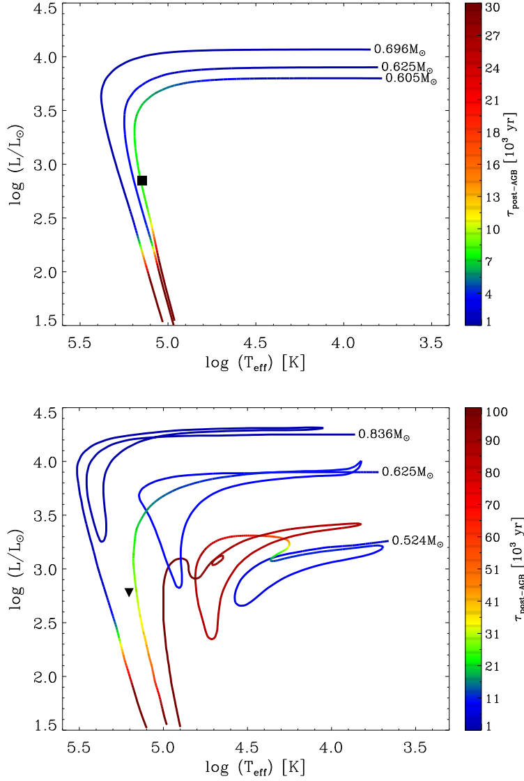
Figure 7.11: Hertzsprung–Russell diagrams for hydrogen-burning models (top panel) with (M_{\text{ZAMS}}, M_\star) = (3M_\odot, 0.605M_\odot) , (3M_\odot, 0.625M_\odot) and (4M_\odot, 0.696M_\odot) , and helium-burning models (bottom panel) with (M_{\text{ZAMS}}, M_\star) = (1M_\odot, 0.524M_\odot) , (3M_\odot, 0.625M_\odot) and (5M_\odot, 0.836M_\odot) from Blöcker (1995a) compared to the position of the central star of SuWt 2 derived from two different photoionization models, namely Model 1 (denoted by ■) and Model 2 (▼). Bottom panel: the evolutionary tracks contain the first evolutionary phase, the VLTP (born-again scenario), and the second evolutionary phase. The colour scales indicate the post-AGB ages ( \tau_{\text{post-AGB}} ) in units of 10^3 \text{ yr} .
