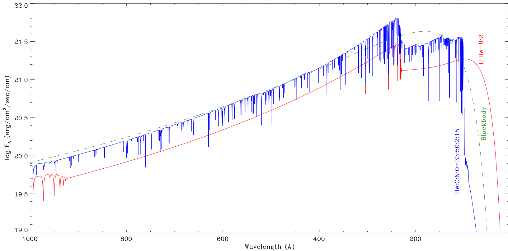
Figure 7.9: Comparison of two NLTE model atmosphere fluxes (Rauch 2003) used as ionizing inputs in our 2 models. Red line: H-rich model with an abundance ratio of \text{H}:\text{He} = 8:2 by mass, \log g = 7 (cgs) and T_{\text{eff}} = 140\,000 K; blue line: PG 1159 model with \text{He}:\text{C}:\text{N}:\text{O} = 33:50:2:15 , \log g = 7 and T_{\text{eff}} = 160\,000 K; and dashed gray green line: the flux of a blackbody with T_{\text{eff}} = 160\,000 K.
