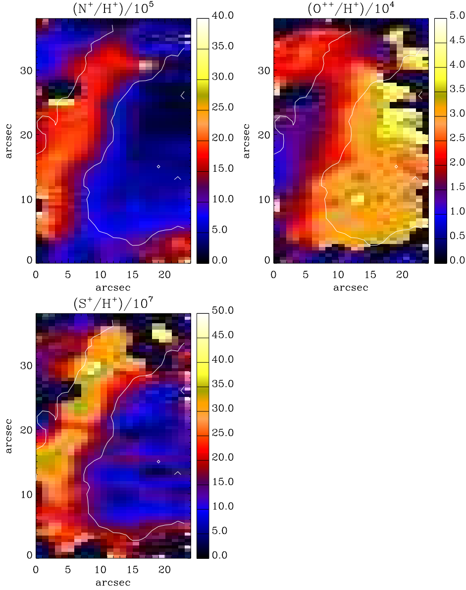
Figure 7.7: Spatial distribution maps of ionic nitrogen abundance ratio N^+/H^+ ( \times 10^{-5} ) from [N\ II] CELs (6548, 6584); ionic oxygen abundance ratio O^{++}/H^+ ( \times 10^{-4} ) from [O\ III] CELs (4959, 5007); and ionic sulfur abundance ratio S^+/H^+ ( \times 10^{-7} ) from [S\ II] CELs (6716, 6731) for T_e = 10000\text{K} and N_e = 100\text{cm}^{-3} . White contour lines show the distribution of the narrow-band emission of H\alpha and [N\ II] in arbitrary unit taken with the ESO 3.6-m telescope.
