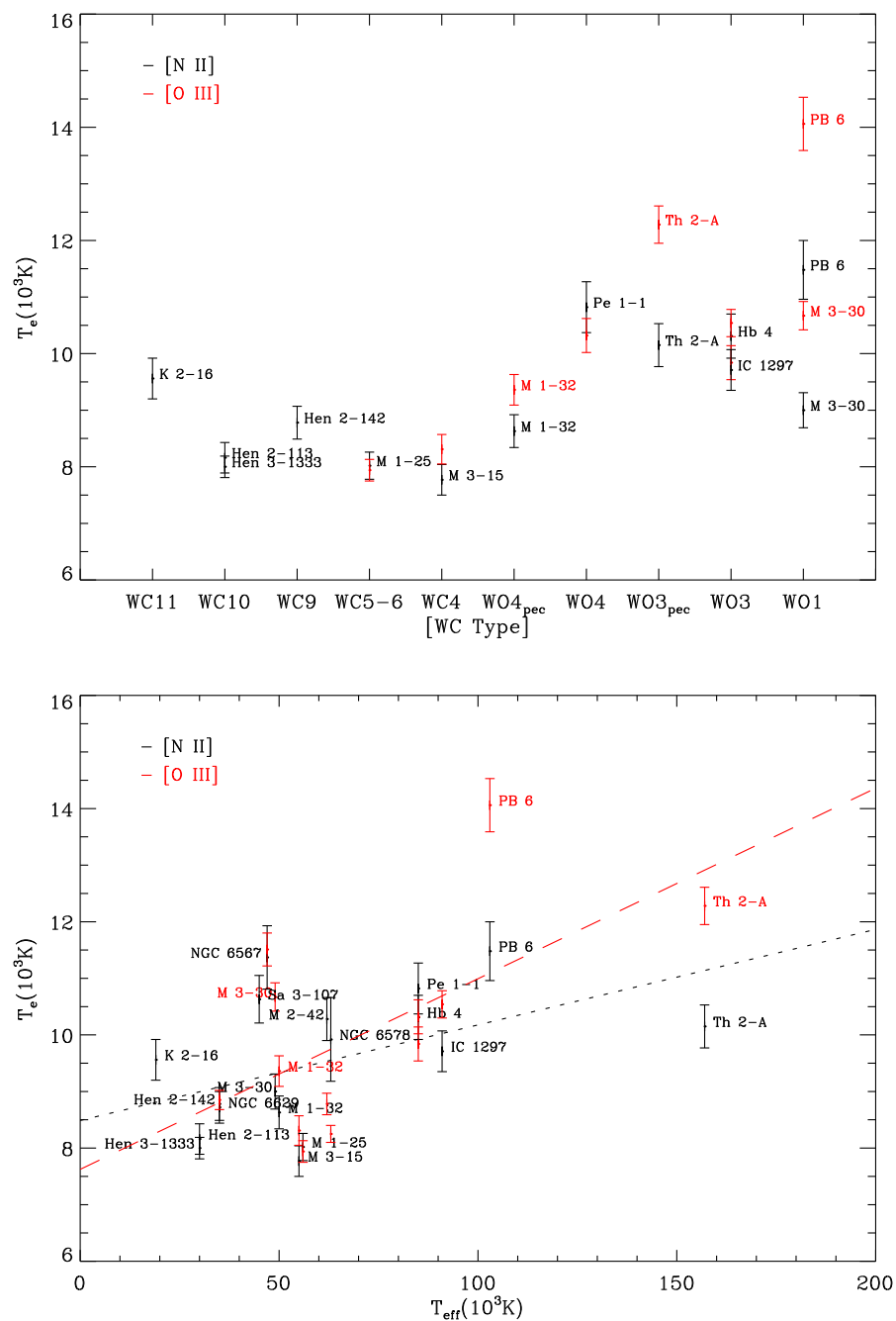
Figure 3.6: Top panel: variation of the electron temperature T_e(10^3 \text{ K}) along the spectral sequence. Bottom panel: variation of the electron temperature T_e(10^3 \text{ K}) along the stellar effective temperature T_{\text{eff}}(10^3 \text{ K}) . The electron temperature derived from [N II] (black line) and [O III] diagnostic ratios (red line). The dotted and dashed lines are respectively linear fits to T_e(\text{[N II]}) and T_e(\text{[O III]}) as functions of T_{\text{eff}} , discussed in the text.
