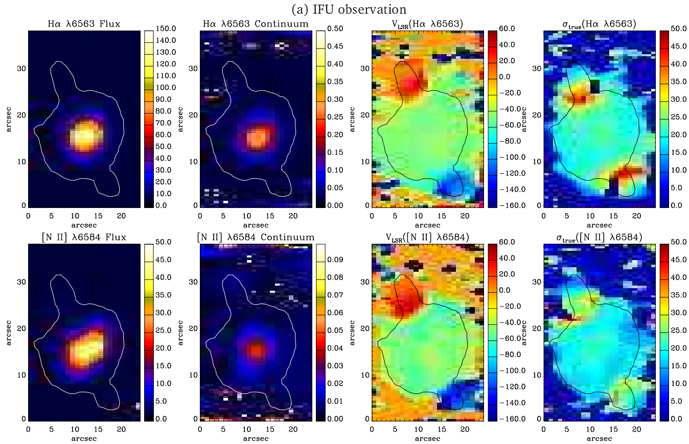
Figure A.3: (a) As Figure A.1 but for Hb4. (b) The SHAPE mesh model before rendering at the best-fitting inclination, two different orientations (inclination: 90^\circ and 0^\circ , respectively), and corresponding rendered model. (c) The HST images taken by F658N filters (Observing program 6347; PI. Borkowski, 1996). (d) The normalized synthetic intensity and radial velocity maps produced by the model.
