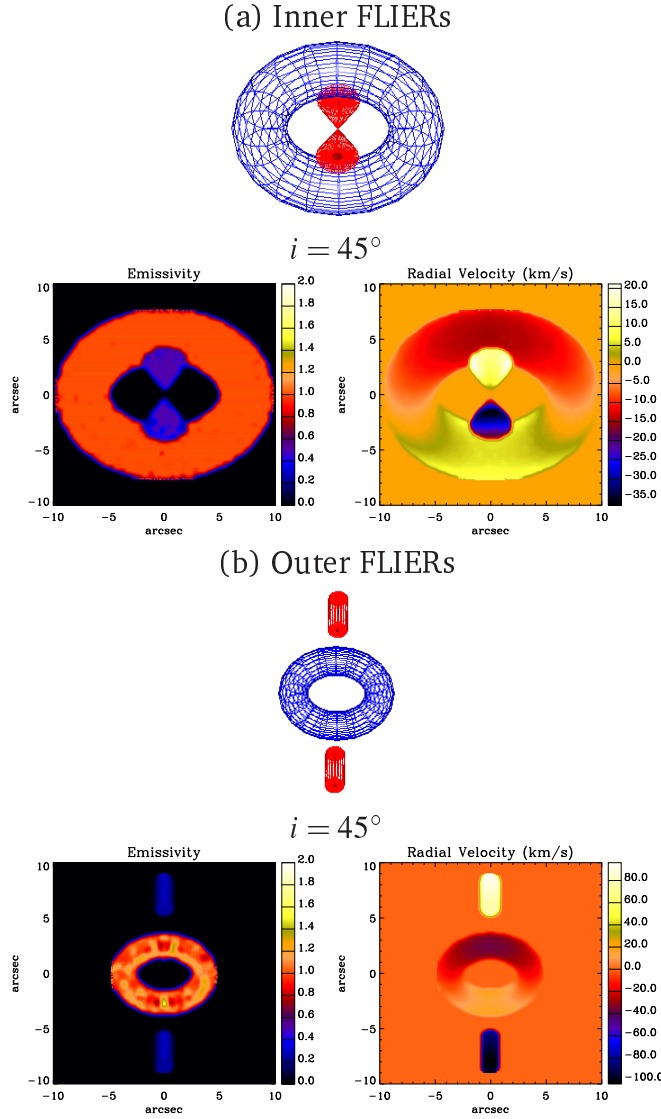
Figure 2.5: The SHAPE mesh models of (a) torus with inner FLIERs and (b) torus with outer FLIERs. The derived 2-D line-of-sight velocity map and the projected 3-D emissivity on the plane of the sky at the inclination of 45^\circ .
