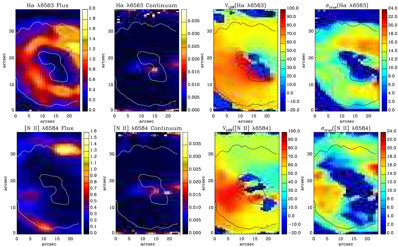
Figure 5.2: Maps of the PN Abell 48 in H \alpha \lambda 6563 Å (top) and [N II] \lambda 6584 Å (bottom) from the IFU (PA = 0°) taken in 2010 April. From left to right: spatial distribution maps of flux intensity, continuum, LSR velocity and velocity dispersion. Flux unit is in 10^{-15} \text{ erg s}^{-1} \text{ cm}^{-2} \text{ spaxel}^{-1} , continuum in 10^{-15} \text{ erg s}^{-1} \text{ cm}^{-2} \text{ Å}^{-1} \text{ spaxel}^{-1} , and velocities in \text{km s}^{-1} . North is up and east is towards the left-hand side. The white/black contour lines show the distribution of the narrow-band emission of H \alpha in arbitrary unit obtained from the SHS.
