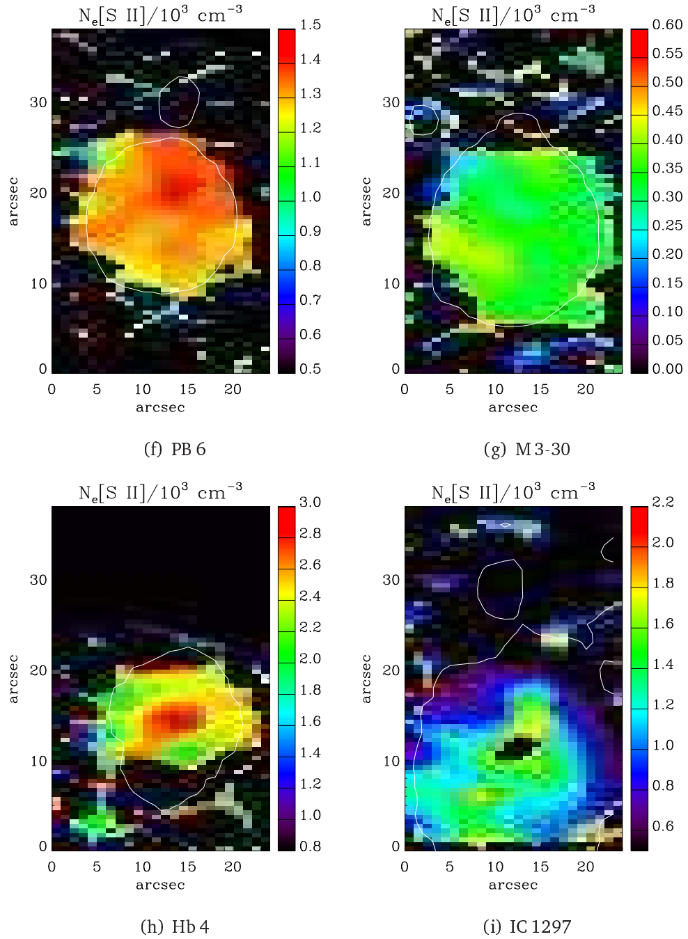
Figure 3.3: As Figure 3.2 but for spatial distribution maps of electron density N_e/10^3 \text{ (cm}^{-3}\text{)} from the flux ratio [S \text{ II}] \text{ } 6717/6731 . The white contour lines show the distribution of the narrow-band emission of H\alpha in arbitrary unit obtained from the SHS.
